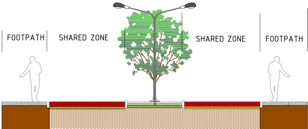
TYPICAL CROSS SECTION OF 'SHARED ZONE' 1:100
