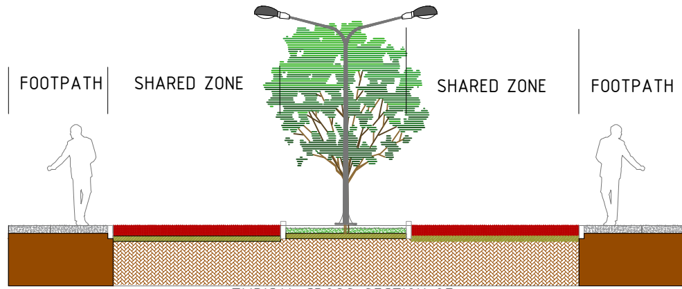
TYPICAL CROSS SECTION OF 'SHARED ZONE' 1:100
