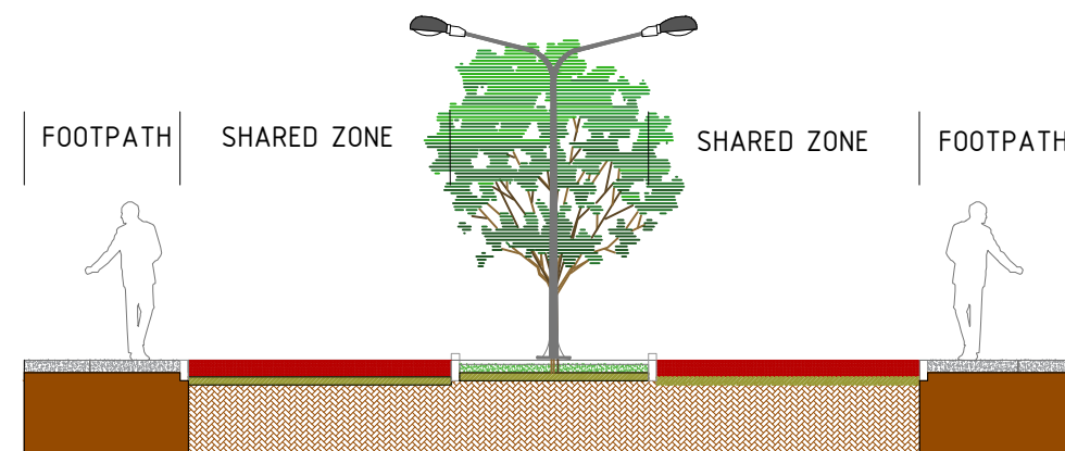
TYPICAL CROSS SECTION OF 'SHARED ZONE'
