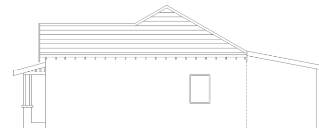
EXISTING ELEVATION 8
