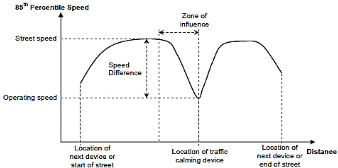
Figure C13 1: Typical speed profile of a traffic-calmed street
