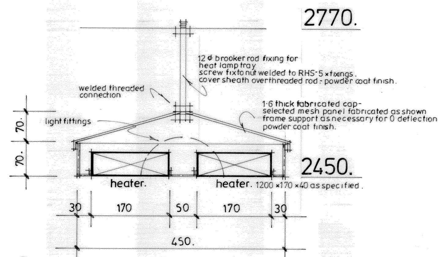
L. SECTION - LIGHTING & HEATING TRAY. 3. SCALE 1:5.
