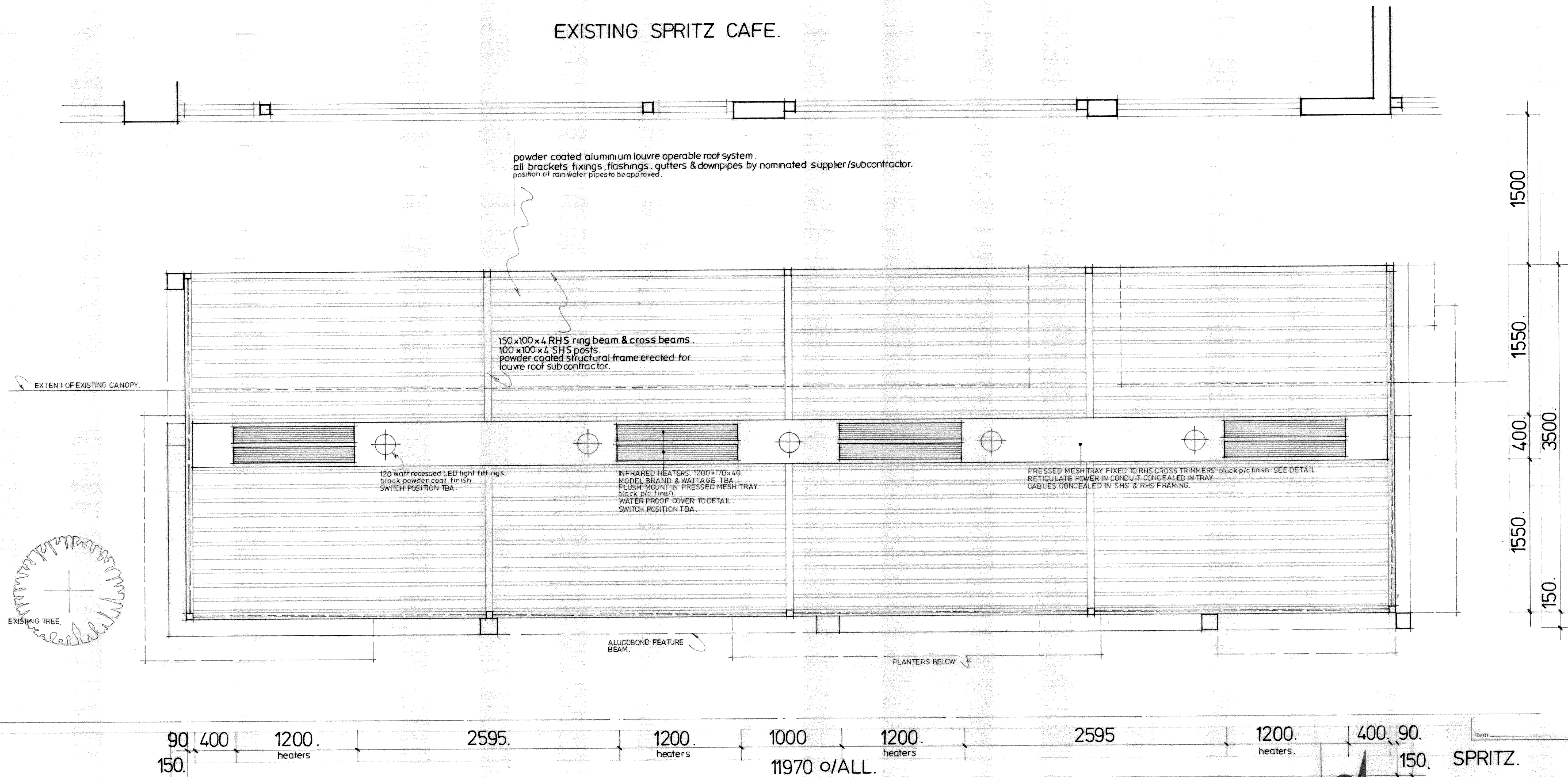
P. 4. CEILING & LIGHTING PLAN. SCALE: 1:20.
